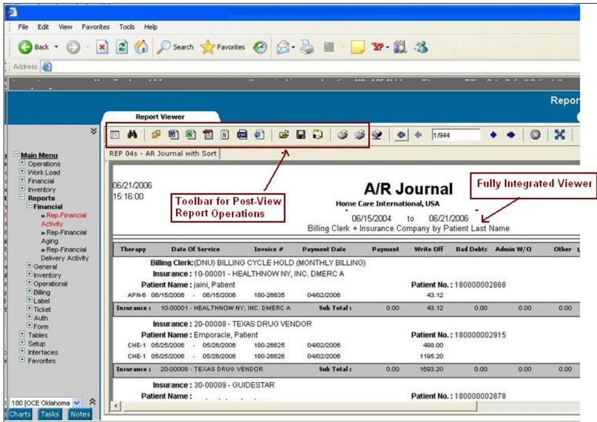
Figure 8: Embedded Report Screen
