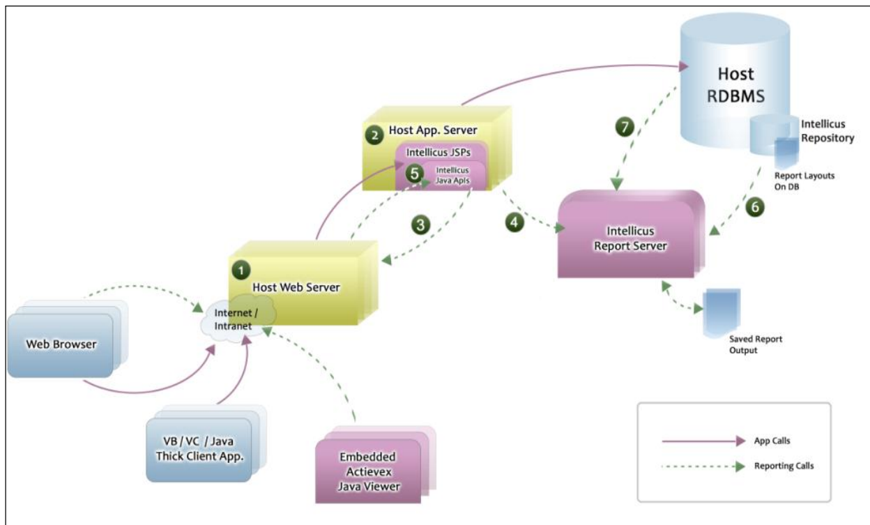
Figure 2: Integrated as embedded in host application
