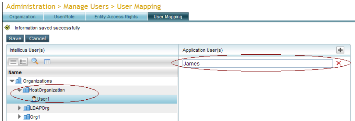
Figure 5: User Mapping
