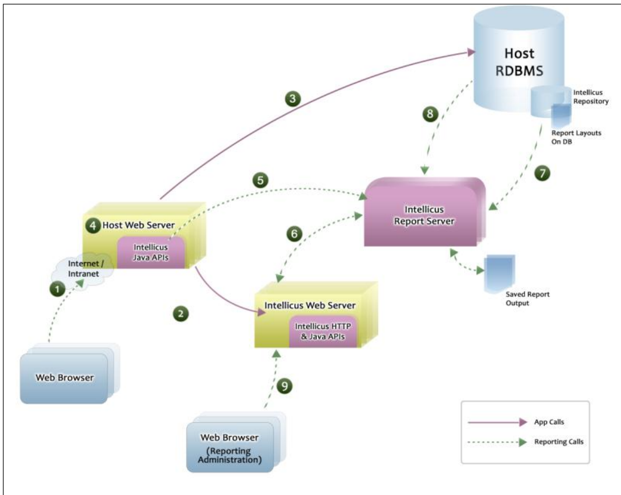
Figure 1: Integrating as a separate portal
